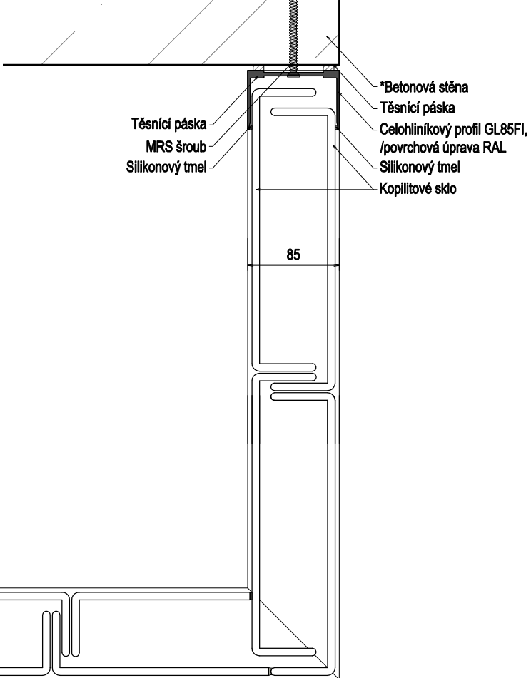
Detail H1.6 (1:5)
